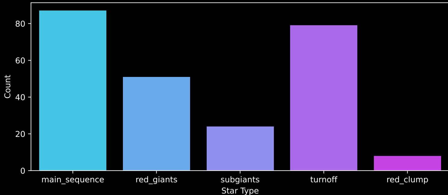
GALAH DR4 Field: [3857] Count plot of Star Type
