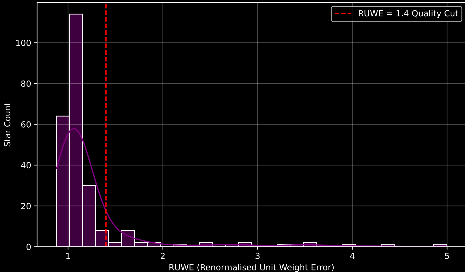
GALAH DR4 Field [3857] RUWE Distribution (n= 243)
